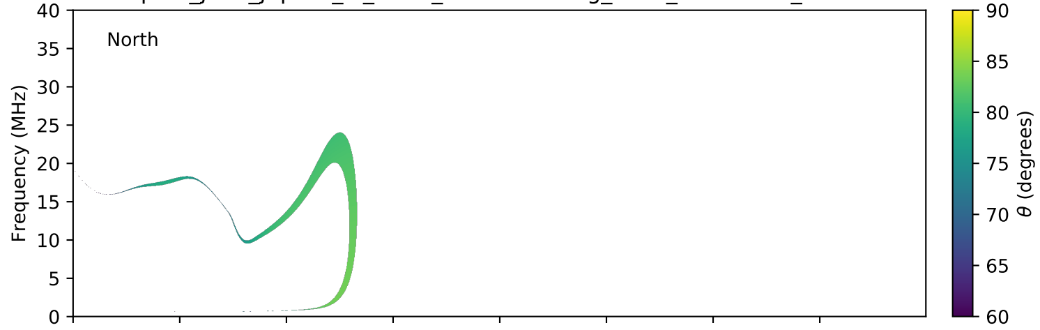
expres_juno_jupiter_io_isaac_lossc-wid1deg_3kev_20181220_v01.cdf
