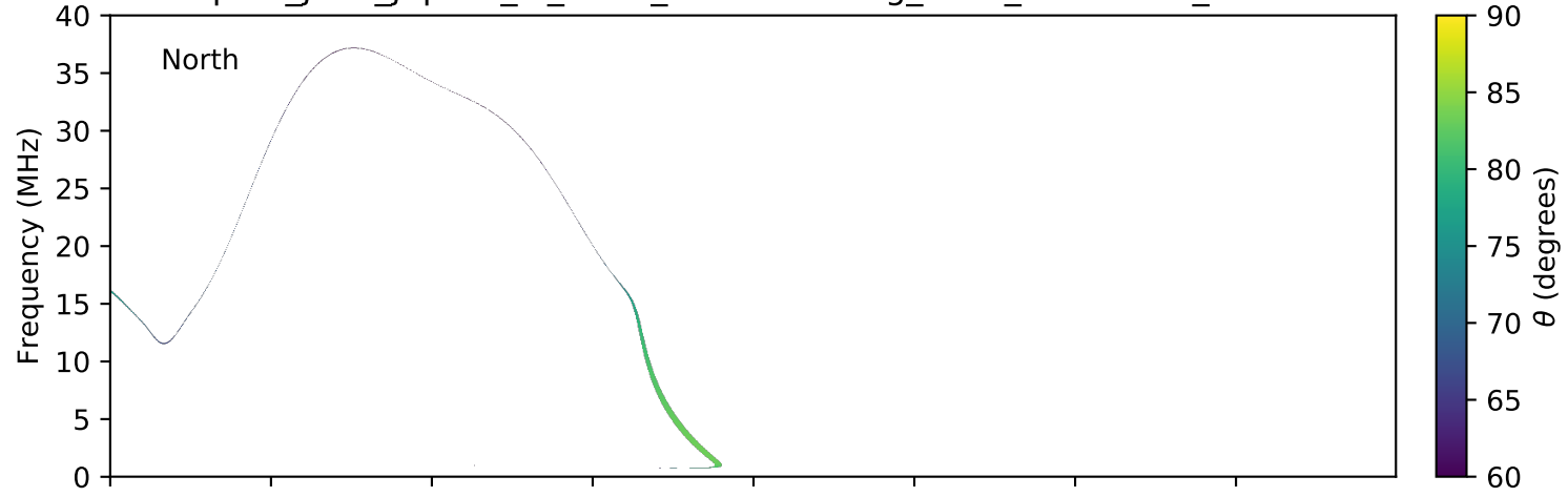
expres_juno_jupiter_io_isaac_lossc-wid1deg_3kev_20181218_v01.cdf
