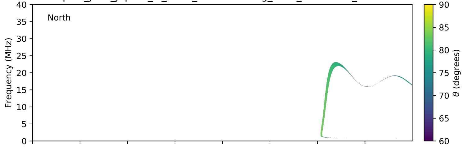
expres_juno_jupiter_io_isaac_lossc-wid1deg_3kev_20181217_v01.cdf
