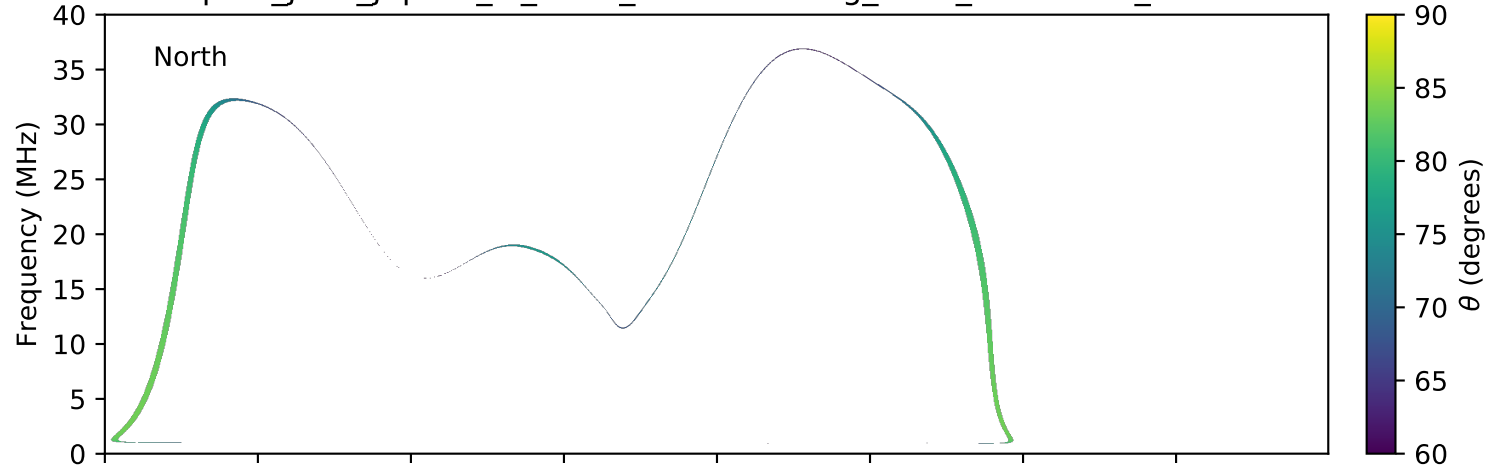
expres_juno_jupiter_io_isaac_lossc-wid1deg_3kev_20181216_v01.cdf
