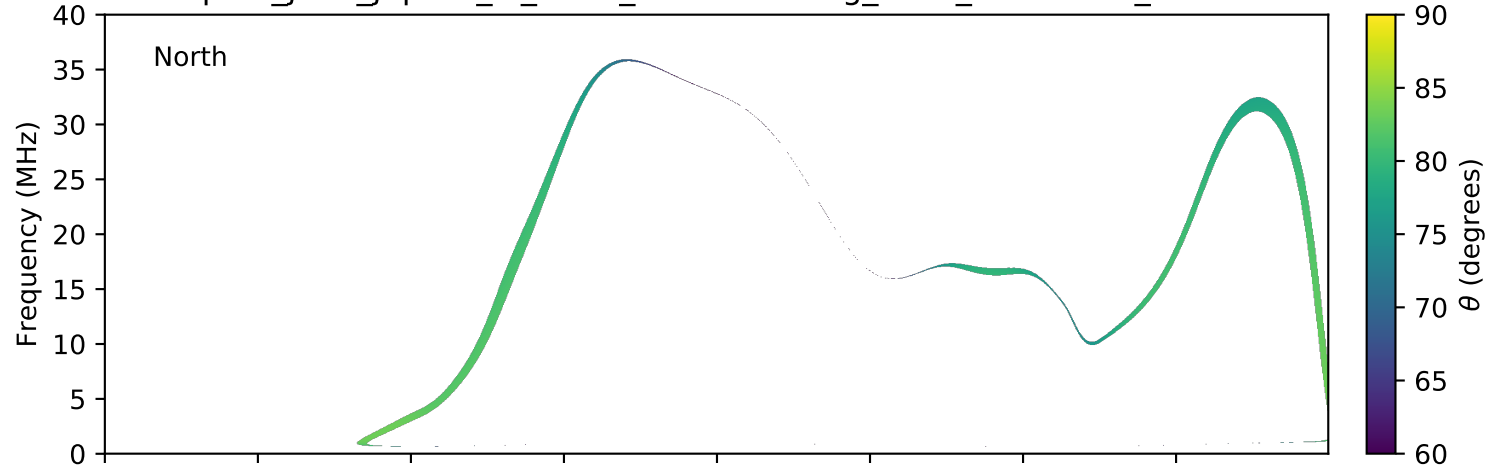
expres_juno_jupiter_io_isaac_lossc-wid1deg_3kev_20181214_v01.cdf
