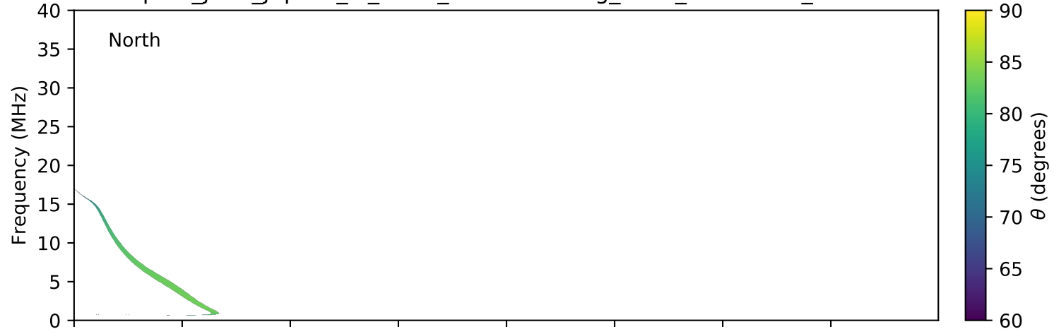
expres_juno_jupiter_io_isaac_lossc-wid1deg_3kev_20181213_v01.cdf
