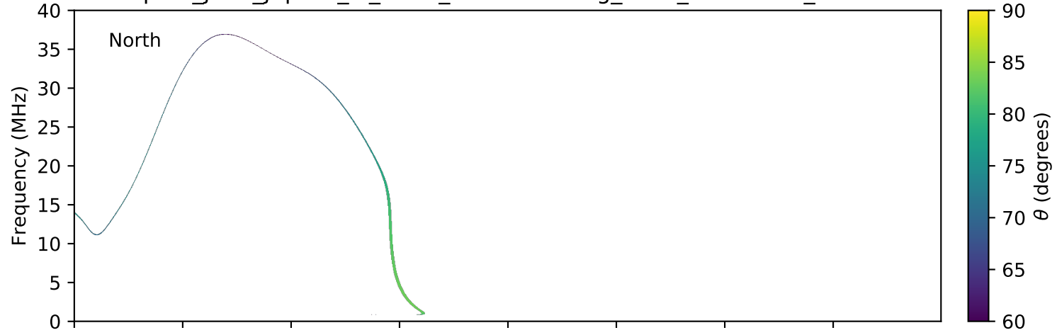
expres_juno_jupiter_io_isaac_lossc-wid1deg_3kev_20181211_v01.cdf
