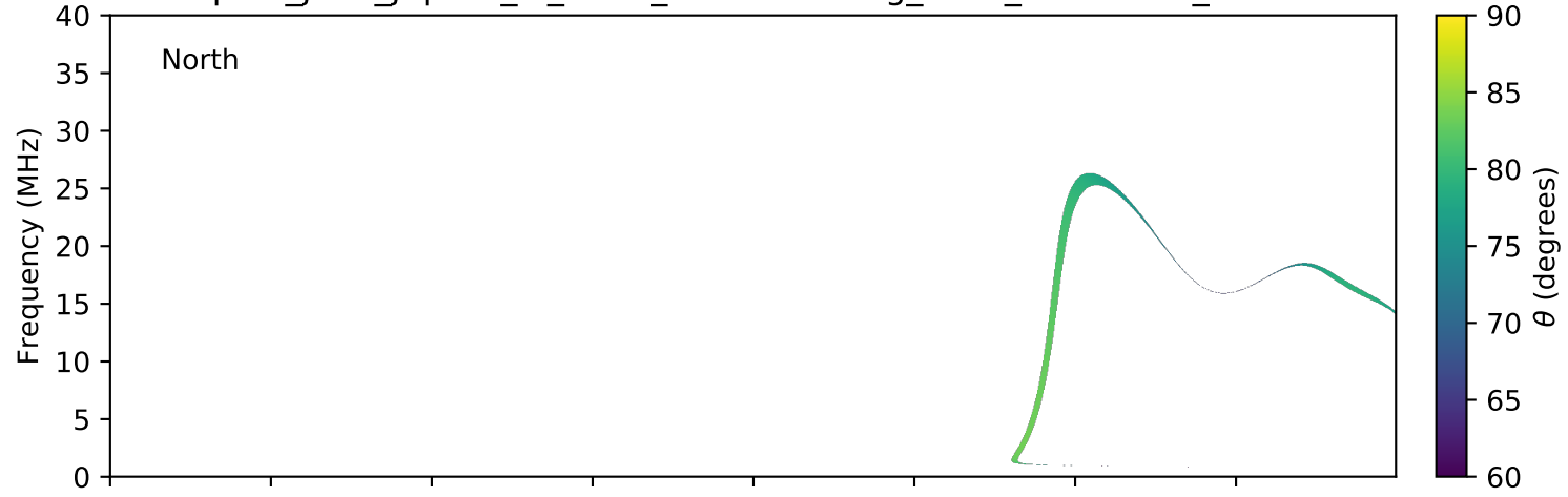
expres_juno_jupiter_io_isaac_lossc-wid1deg_3kev_20181210_v01.cdf
