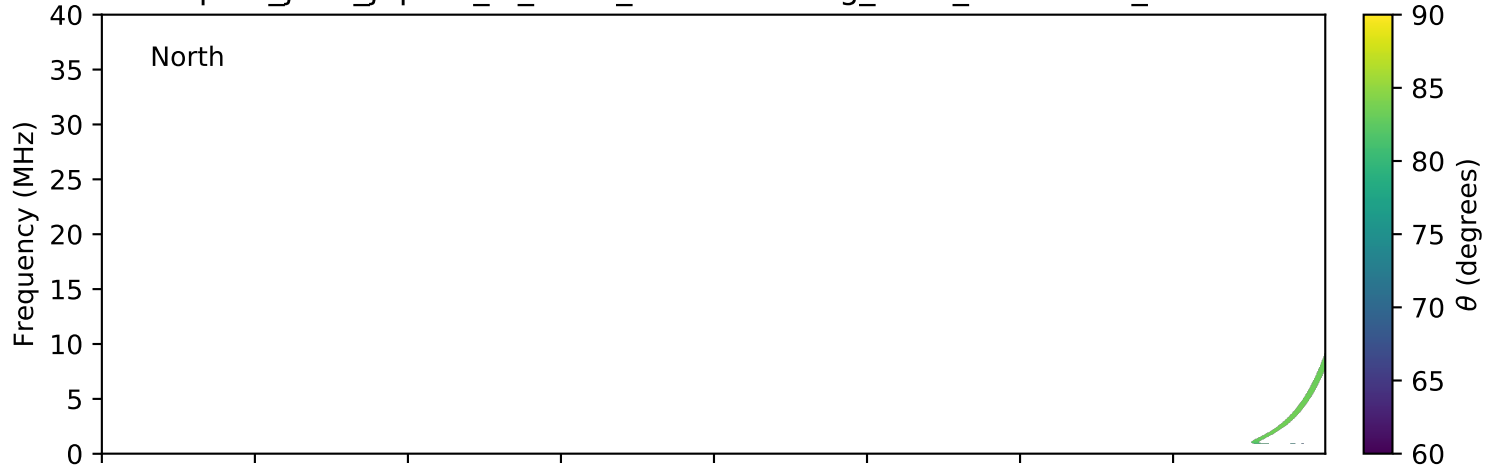
expres_juno_jupiter_io_isaac_lossc-wid1deg_3kev_20181208_v01.cdf
