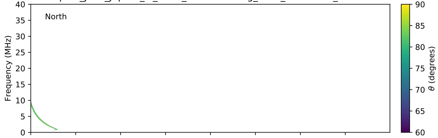
expres_juno_jupiter_io_isaac_lossc-wid1deg_3kev_20181206_v01.cdf
