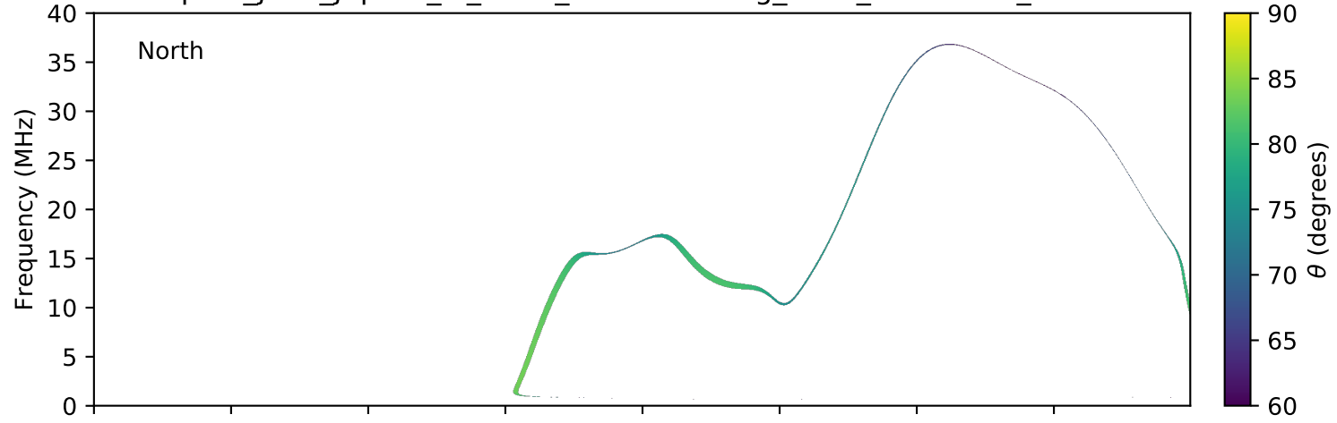
expres_juno_jupiter_io_isaac_lossc-wid1deg_3kev_20181205_v01.cdf
