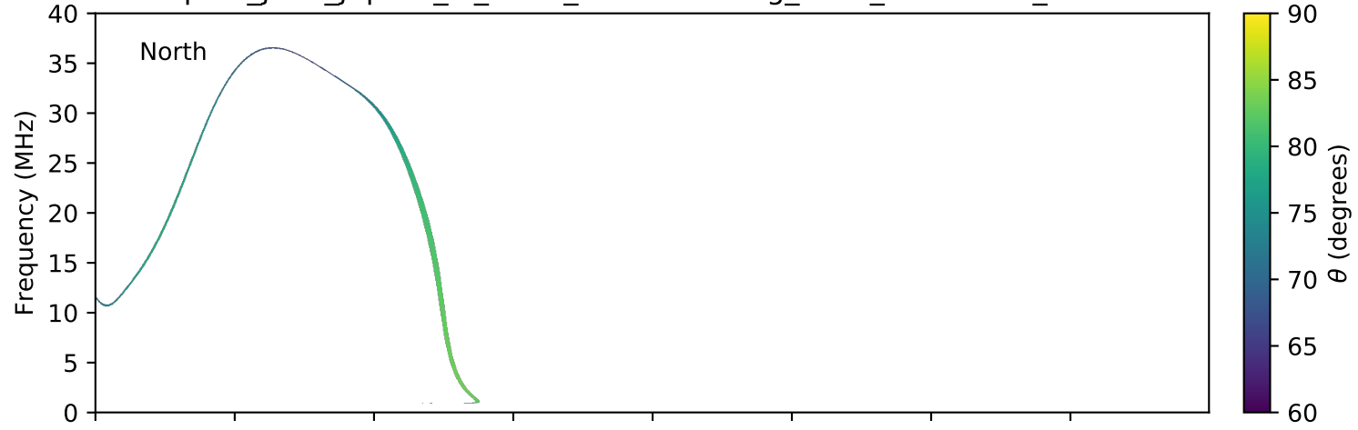
expres_juno_jupiter_io_isaac_lossc-wid1deg_3kev_20181204_v01.cdf
