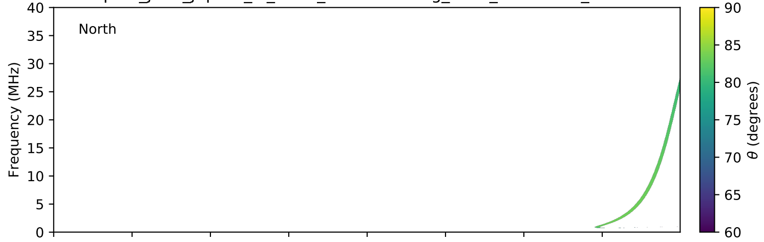
expres_juno_jupiter_io_isaac_lossc-wid1deg_3kev_20181201_v01.cdf
