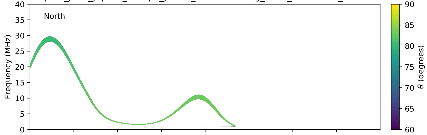
expres_juno_jupiter_europa_jrm09_lossc-wid1deg_3kev_20181231_v01.cdf
