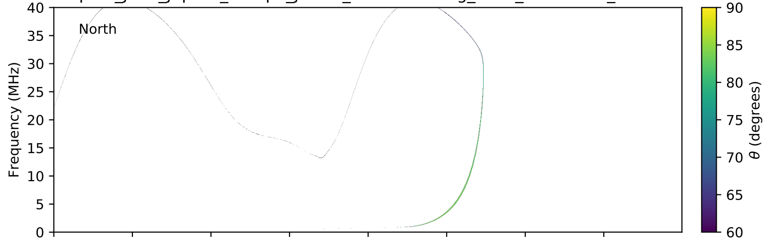
expres_juno_jupiter_europa_jrm09_lossc-wid1deg_3kev_20181221_v01.cdf
