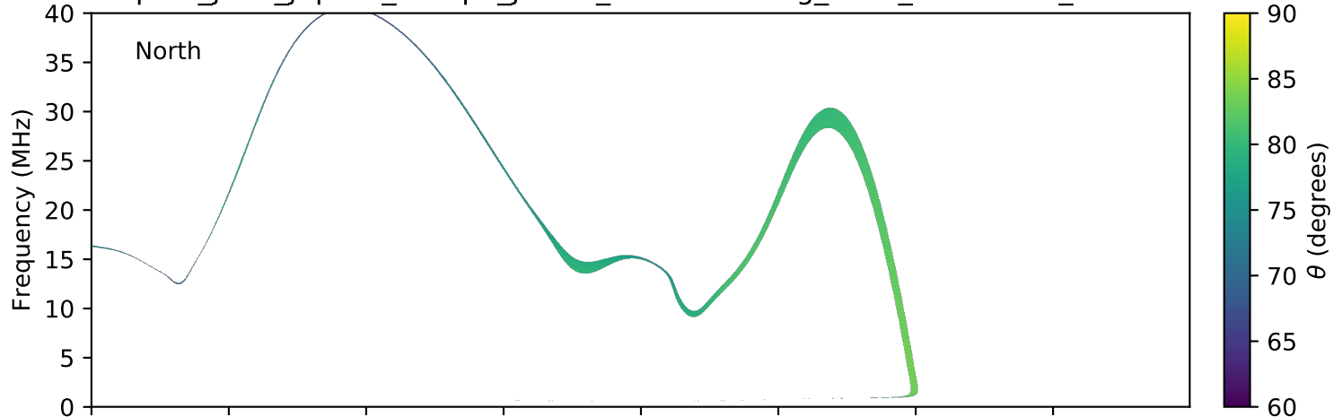
expres_juno_jupiter_europa_jrm09_lossc-wid1deg_3kev_20181218_v01.cdf
