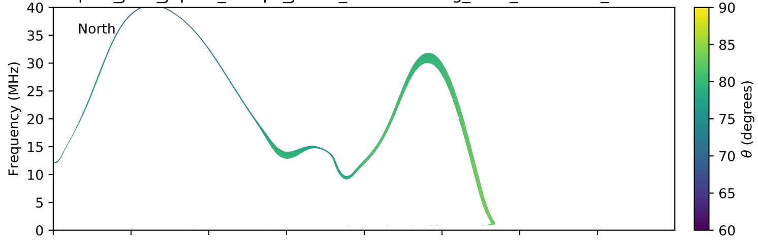
expres_juno_jupiter_europa_jrm09_lossc-wid1deg_3kev_20181216_v01.cdf
