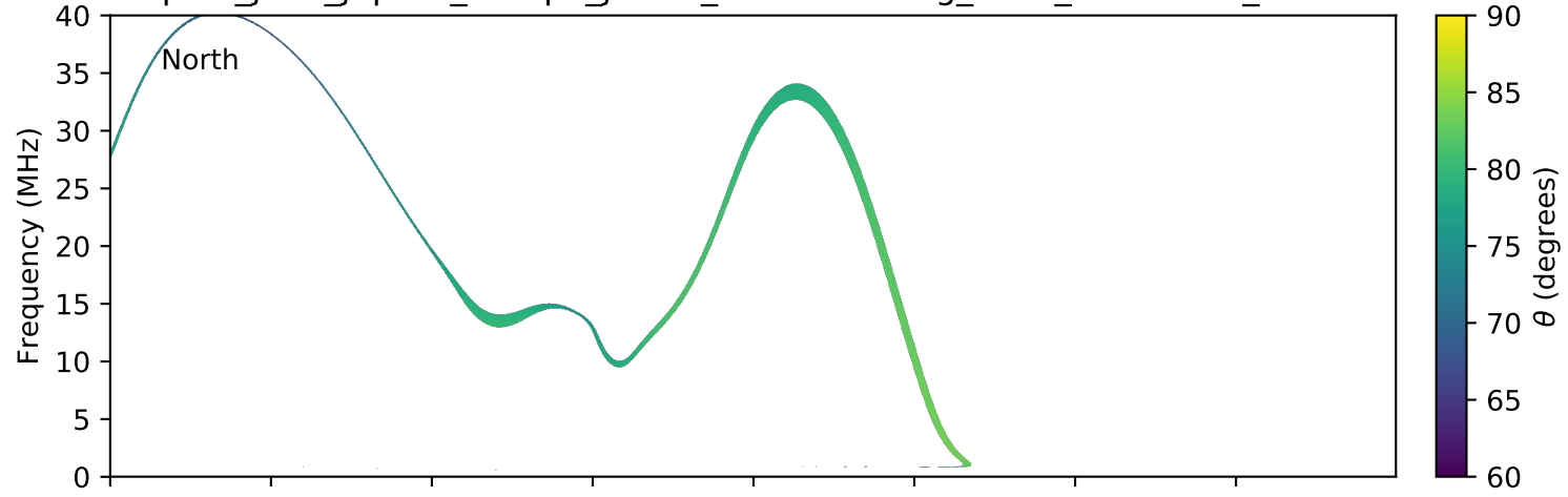
expres_juno_jupiter_europa_jrm09_lossc-wid1deg_3kev_20181214_v01.cdf
