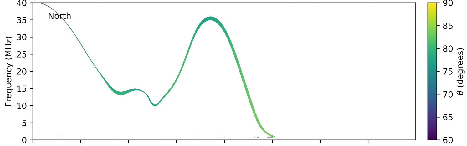
expres_juno_jupiter_europa_jrm09_lossc-wid1deg_3kev_20181212_v01.cdf
