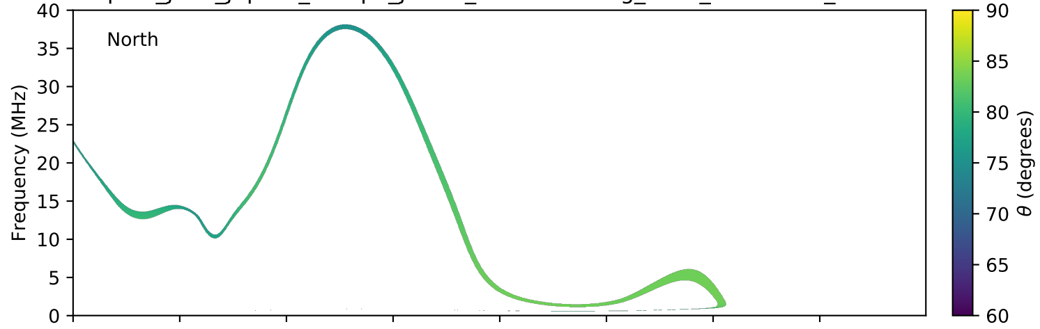
expres_juno_jupiter_europa_jrm09_lossc-wid1deg_3kev_20181208_v01.cdf
