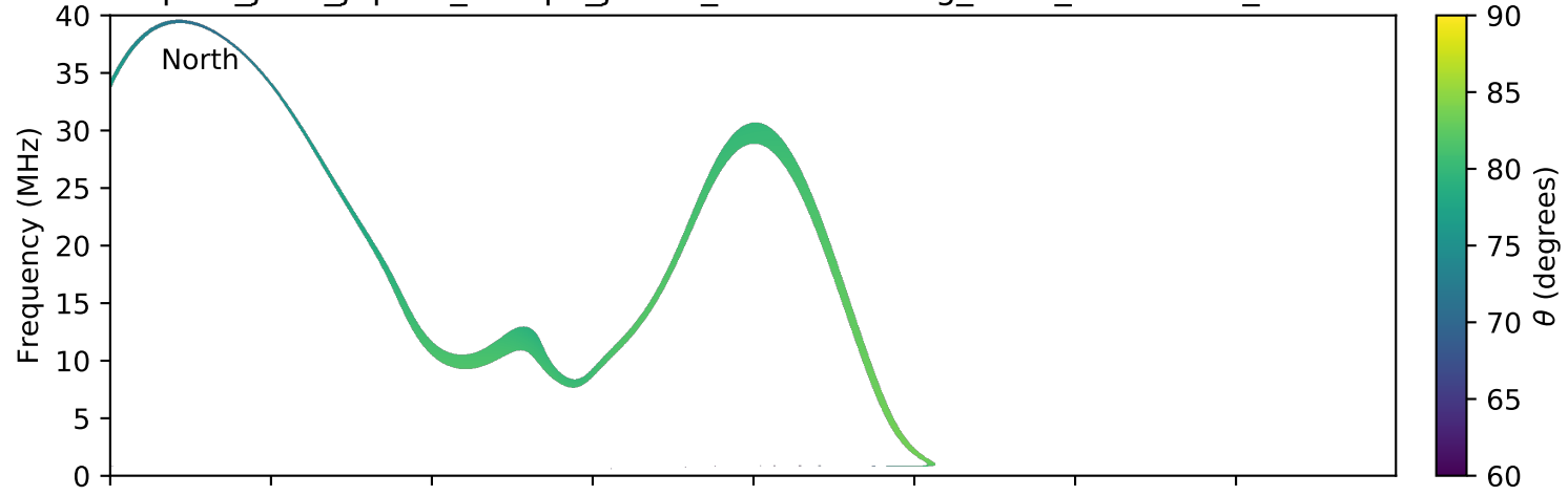
expres_juno_jupiter_europa_jrm09_lossc-wid1deg_3kev_20181207_v01.cdf
