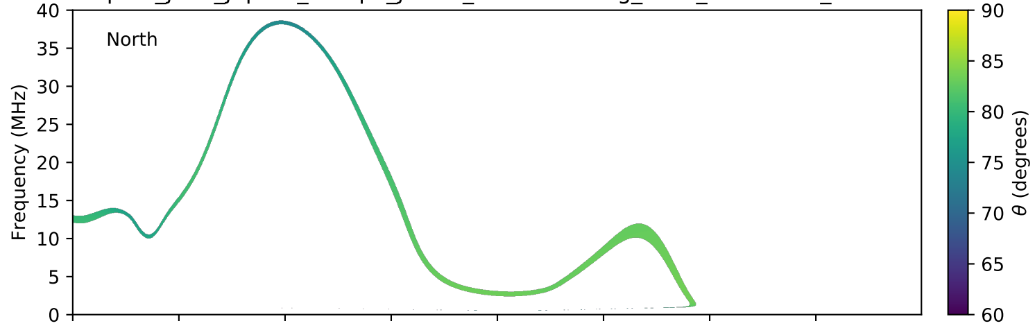
expres_juno_jupiter_europa_jrm09_lossc-wid1deg_3kev_20181206_v01.cdf
