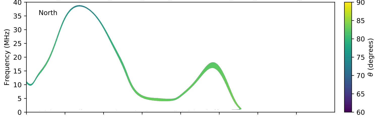
expres_juno_jupiter_europa_jrm09_lossc-wid1deg_3kev_20181204_v01.cdf
