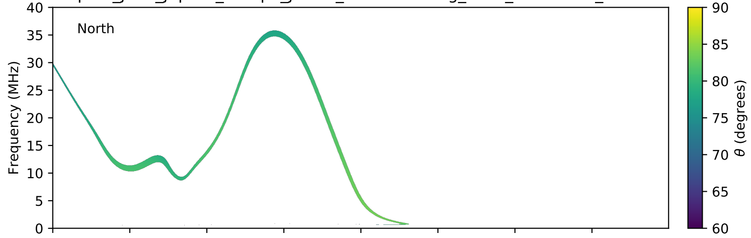
expres_juno_jupiter_europa_jrm09_lossc-wid1deg_3kev_20181203_v01.cdf
