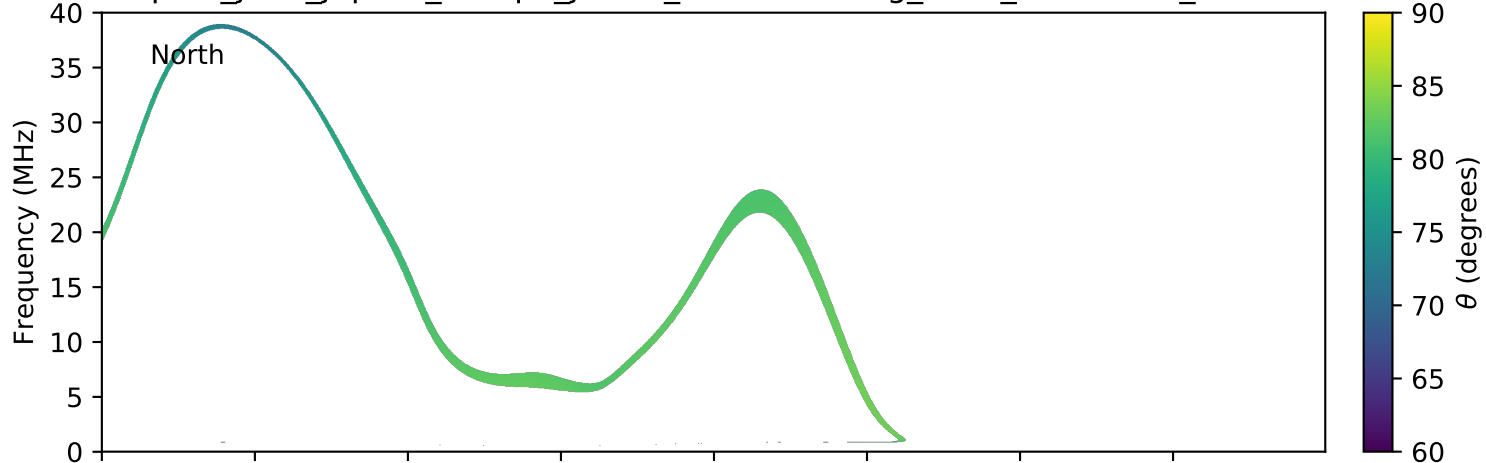
expres_juno_jupiter_europa_jrm09_lossc-wid1deg_3kev_20181202_v01.cdf
