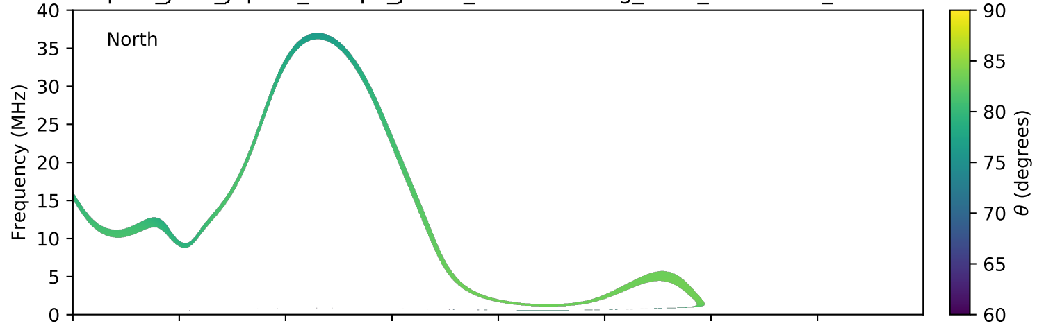
expres_juno_jupiter_europa_jrm09_lossc-wid1deg_3kev_20181201_v01.cdf
