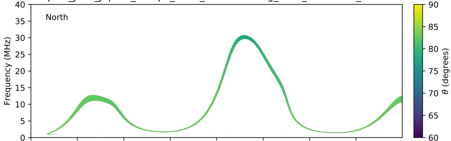
expres_juno_jupiter_europa_isaac_lossc-wid1deg_3kev_20181228_v01.cdf
