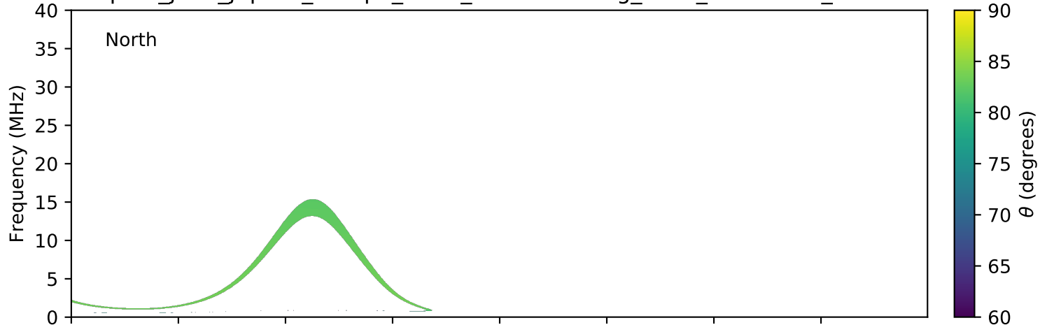
expres_juno_jupiter_europa_isaac_lossc-wid1deg_3kev_20181225_v01.cdf
