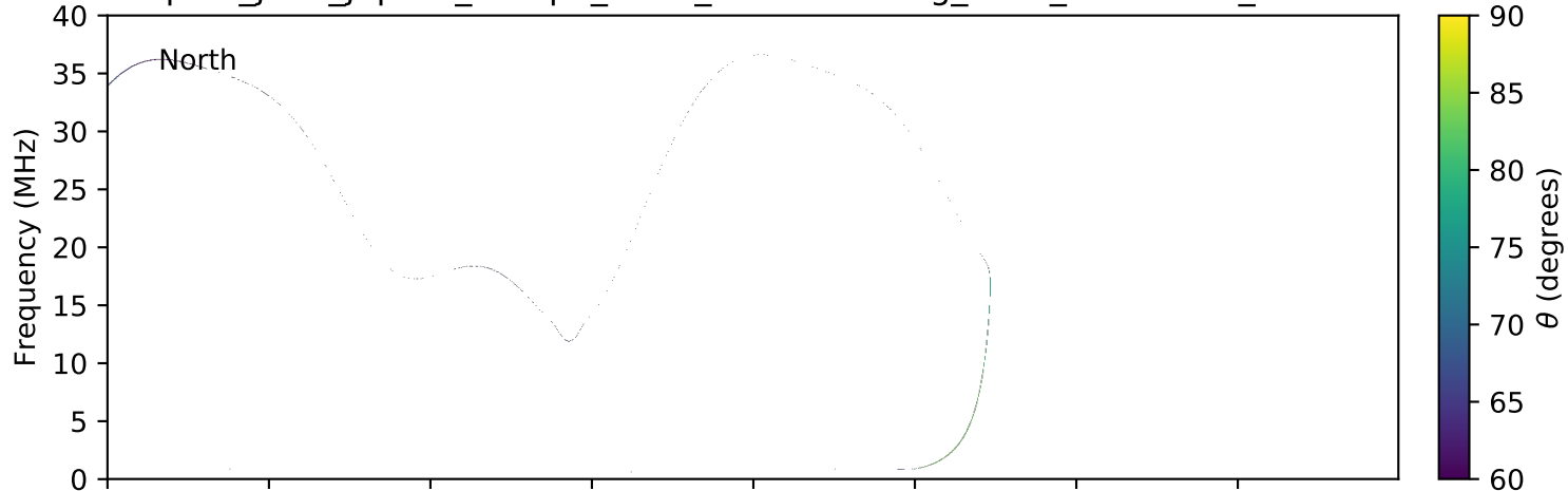
expres_juno_jupiter_europa_isaac_lossc-wid1deg_3kev_20181221_v01.cdf
