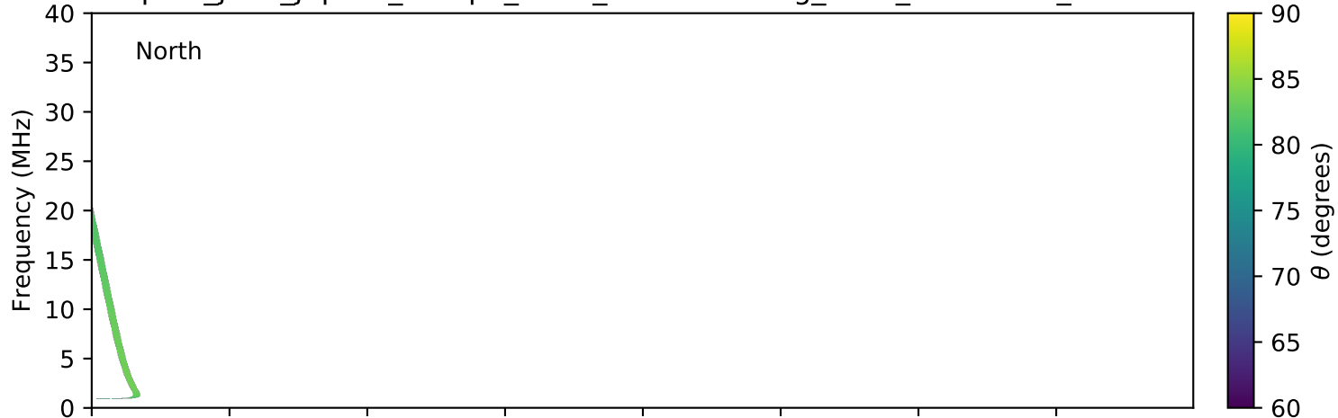
expres_juno_jupiter_europa_isaac_lossc-wid1deg_3kev_20181215_v01.cdf
