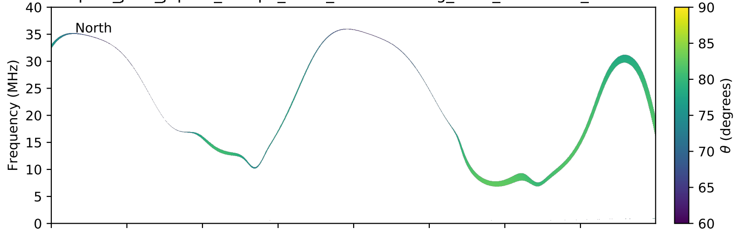
expres_juno_jupiter_europa_isaac_lossc-wid1deg_3kev_20181214_v01.cdf
