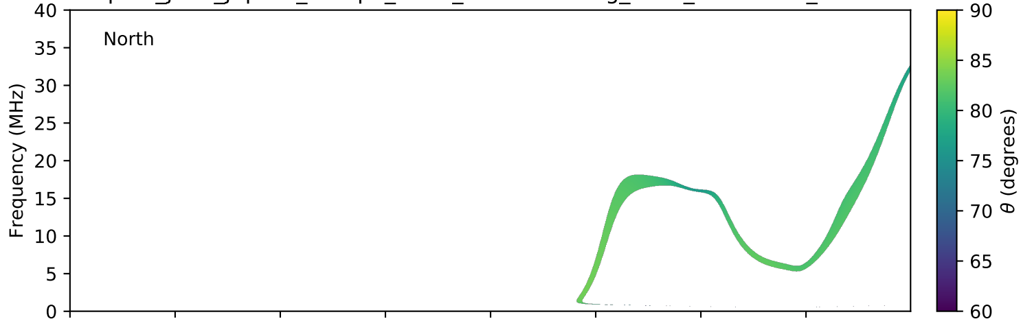
expres_juno_jupiter_europa_isaac_lossc-wid1deg_3kev_20181213_v01.cdf
