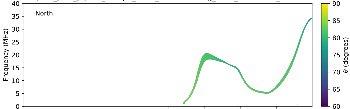
expres_juno_jupiter_europa_isaac_lossc-wid1deg_3kev_20181206_v01.cdf
