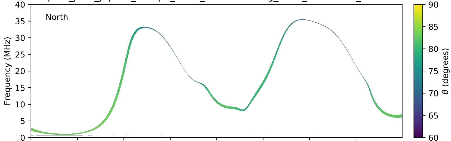
expres_juno_jupiter_europa_isaac_lossc-wid1deg_3kev_20181203_v01.cdf
