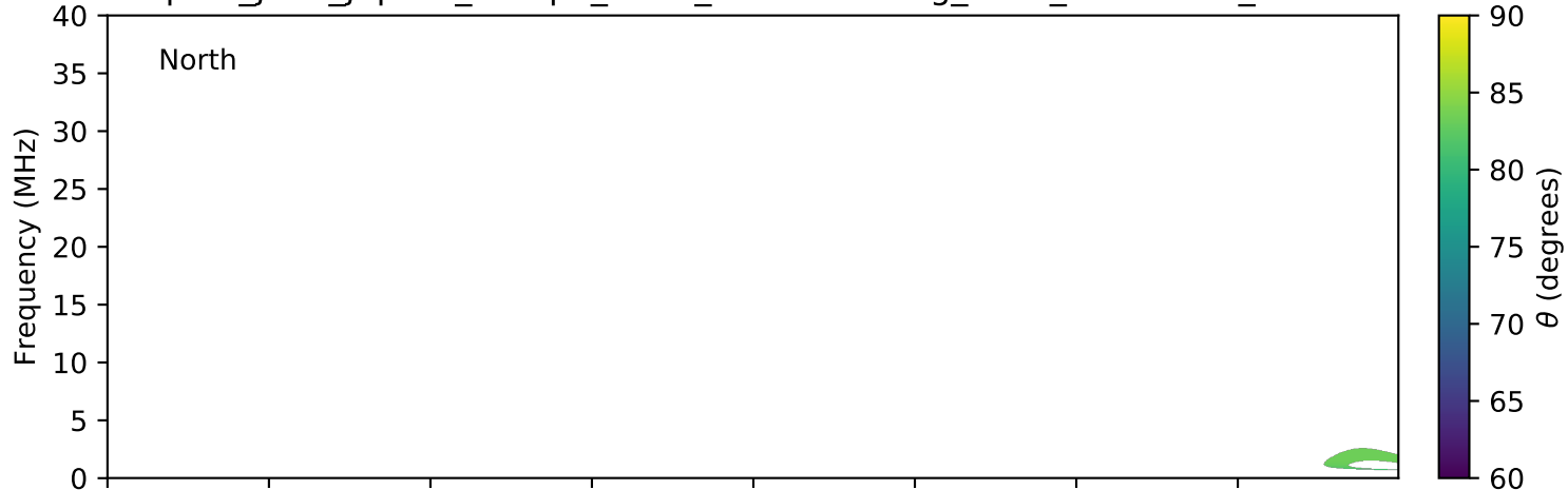
expres_juno_jupiter_europa_isaac_lossc-wid1deg_3kev_20181202_v01.cdf
