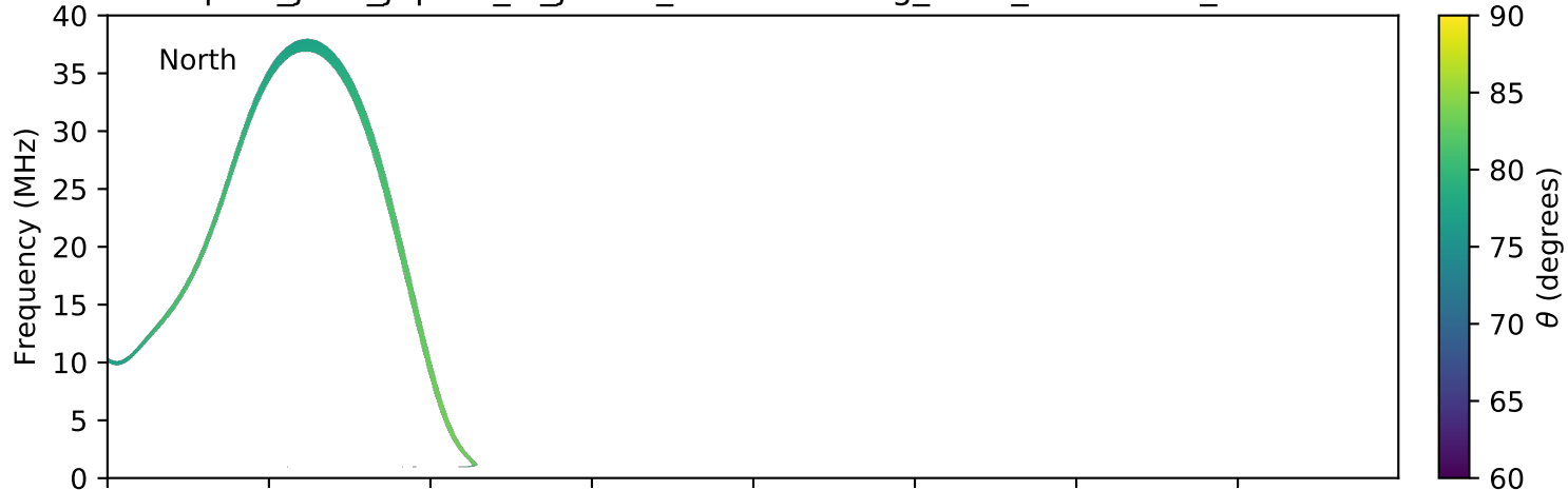
expres_juno_jupiter_io_jrm09_lossc-wid1deg_3kev_20181127_v01.cdf
