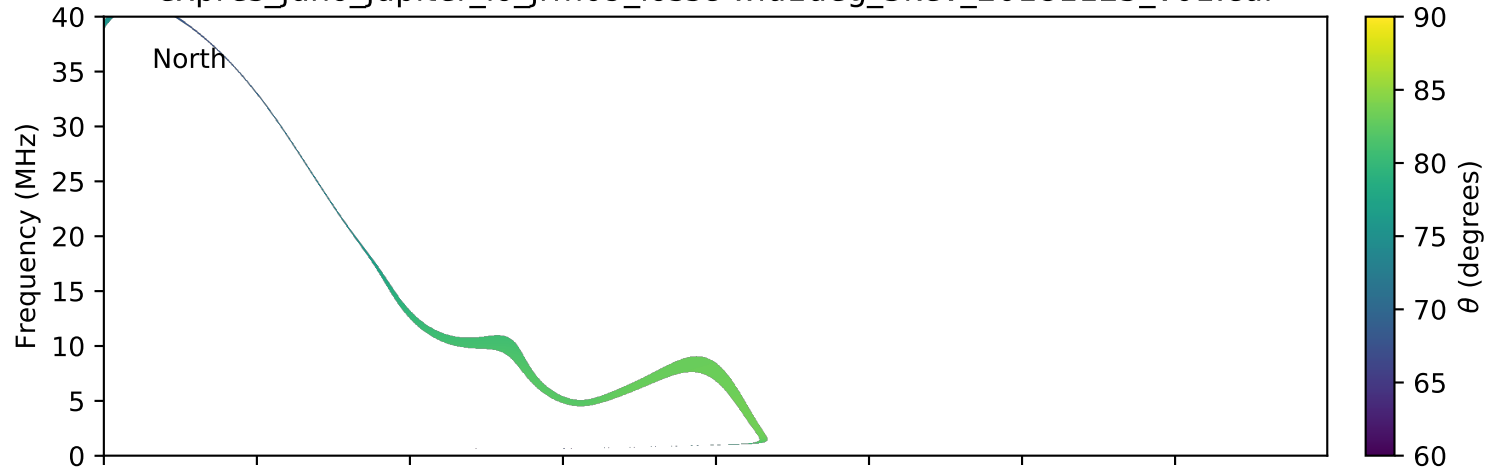
expres_juno_jupiter_io_jrm09_lossc-wid1deg_3kev_20181125_v01.cdf
