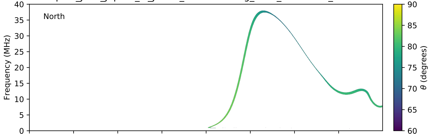
expres_juno_jupiter_io_jrm09_lossc-wid1deg_3kev_20181119_v01.cdf
