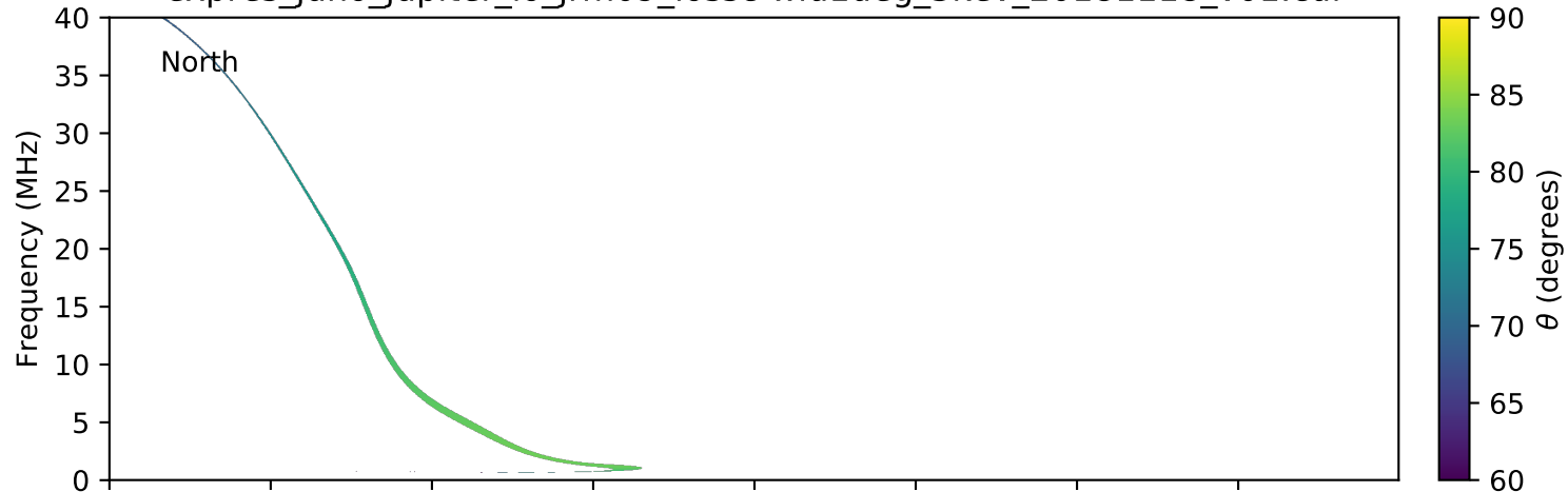
expres_juno_jupiter_io_jrm09_lossc-wid1deg_3kev_20181118_v01.cdf
