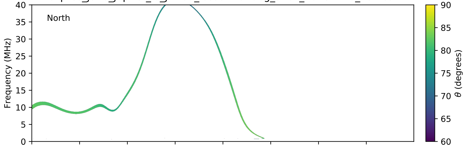
expres_juno_jupiter_io_jrm09_lossc-wid1deg_3kev_20181116_v01.cdf
