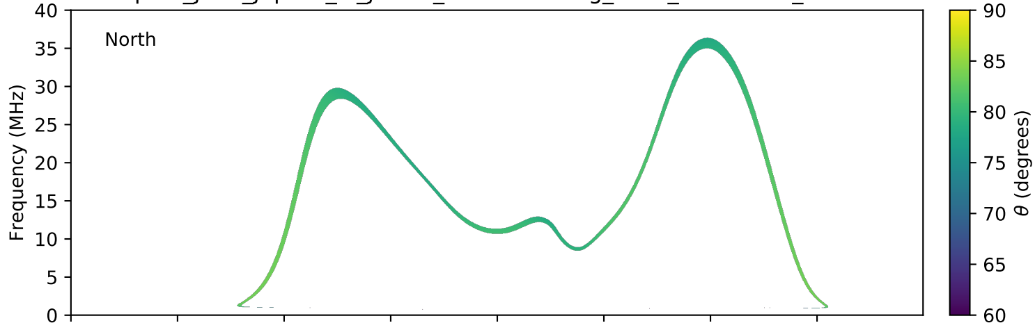
expres_juno_jupiter_io_jrm09_lossc-wid1deg_3kev_20181114_v01.cdf
