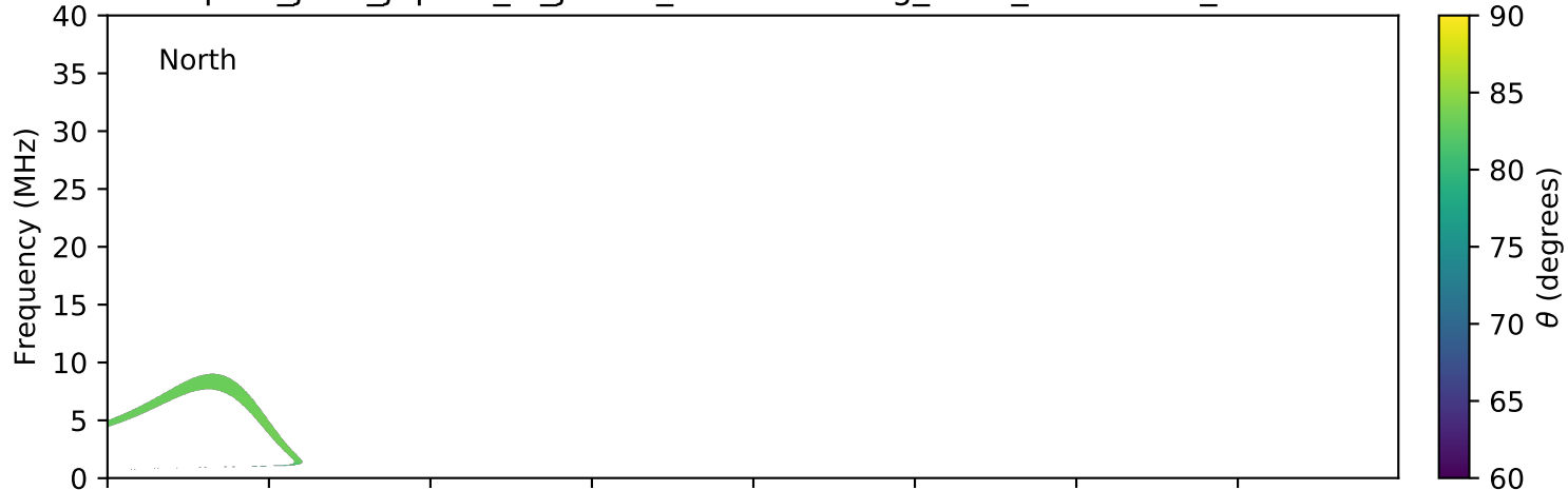
expres_juno_jupiter_io_jrm09_lossc-wid1deg_3kev_20181113_v01.cdf
