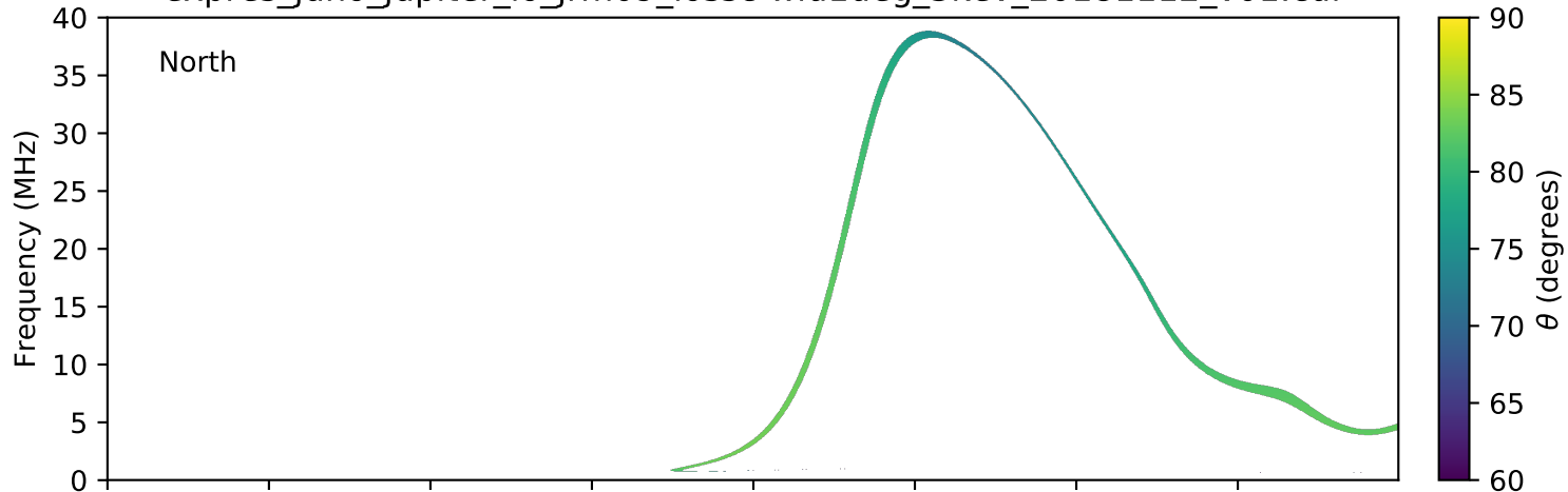
expres_juno_jupiter_io_jrm09_lossc-wid1deg_3kev_20181112_v01.cdf
