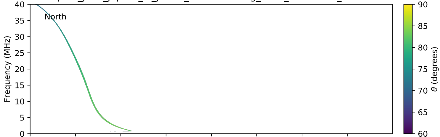
expres_juno_jupiter_io_jrm09_lossc-wid1deg_3kev_20181111_v01.cdf
