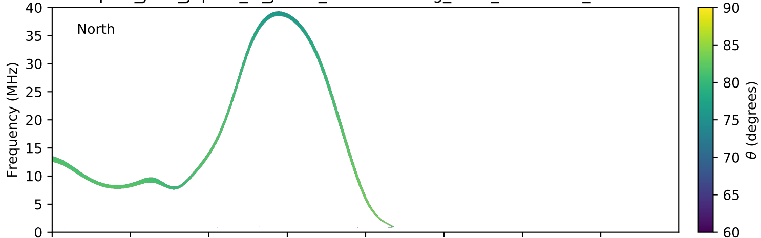
expres_juno_jupiter_io_jrm09_lossc-wid1deg_3kev_20181109_v01.cdf
