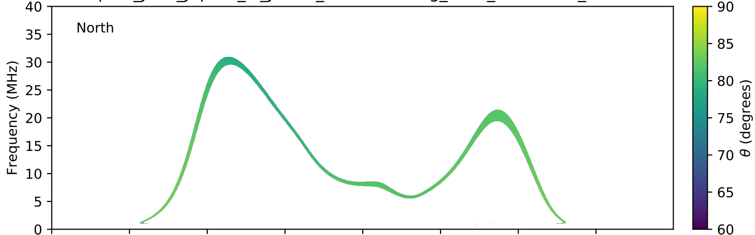
expres_juno_jupiter_io_jrm09_lossc-wid1deg_3kev_20181107_v01.cdf
