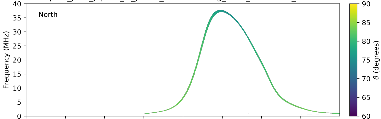
expres_juno_jupiter_io_jrm09_lossc-wid1deg_3kev_20181105_v01.cdf
