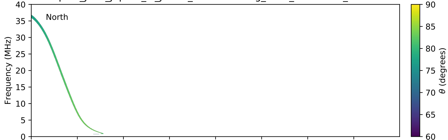
expres_juno_jupiter_io_jrm09_lossc-wid1deg_3kev_20181104_v01.cdf
