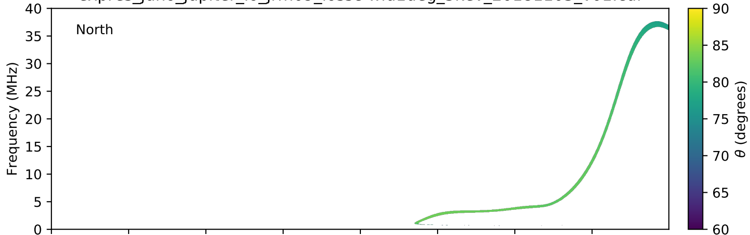
expres_juno_jupiter_io_jrm09_lossc-wid1deg_3kev_20181103_v01.cdf
