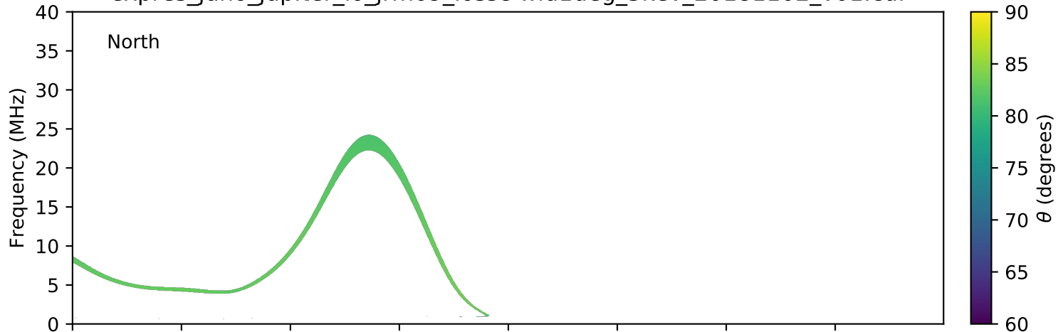
expres_juno_jupiter_io_jrm09_lossc-wid1deg_3kev_20181102_v01.cdf
